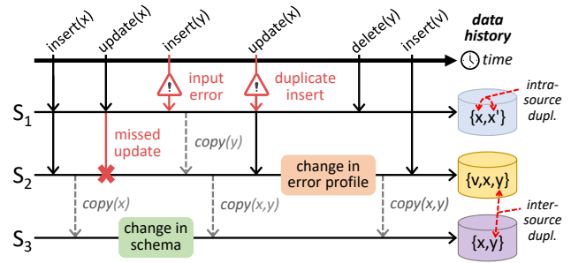
Figure 3: Event-based error model with three data sources. Events are inserts, updates, and deletes of records, copying processes, and changes in the schema and error profiles.
