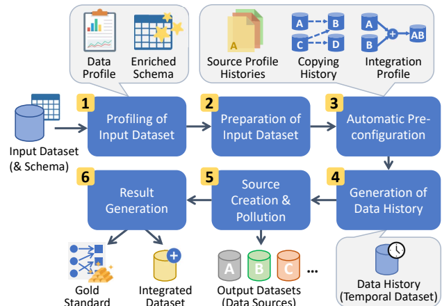
Figure 1: Basic architecture of DaPo +
