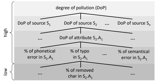
Figure 2: Sample hierarchy of error parameters. Automated mappings from the few abstract high-level parameters to the many low-level parameters support inexperienced users in configuring the actual error probabilities.
